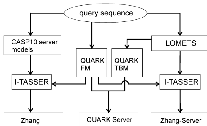
Figure 1. Flowchart for automated structure modeling generated for “Zhang”, “Zhang-Server”, and “QUARK” in CASP10.
