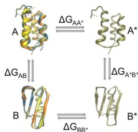
Figure 1: The thermodynamic cycle involving confinement method
