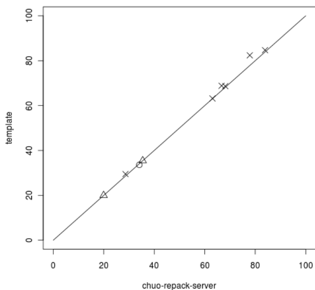
Figure 1. Show the GDT_TS plot of the "template" against the "chuo-repack-server". The superior results of the "chuo-repack-server" are described by the circle, and that of the "template" is described by the cross. The triangle means the same GDT_TS values.
