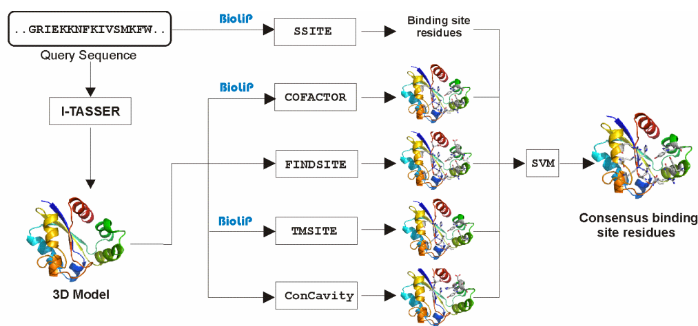
Figure 1. The architecture of COACH for binding sites prediction.
