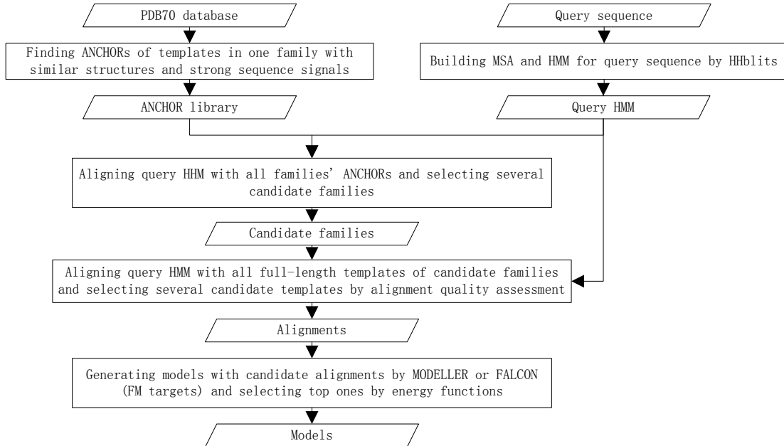
Fig.1 Flowchart of FALCON-TOPO
