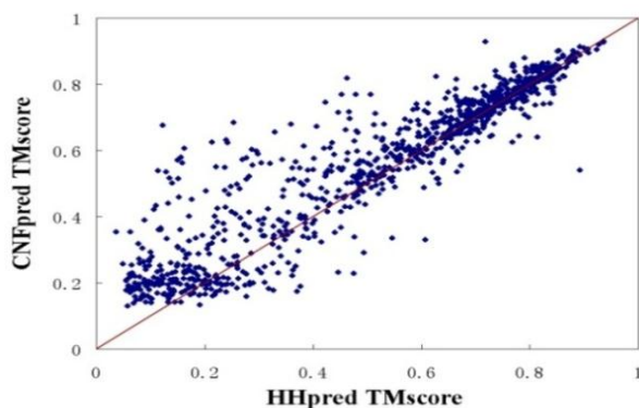
Figure 1. Comparison of RaptorX with HHpred on 1000 proteins.
