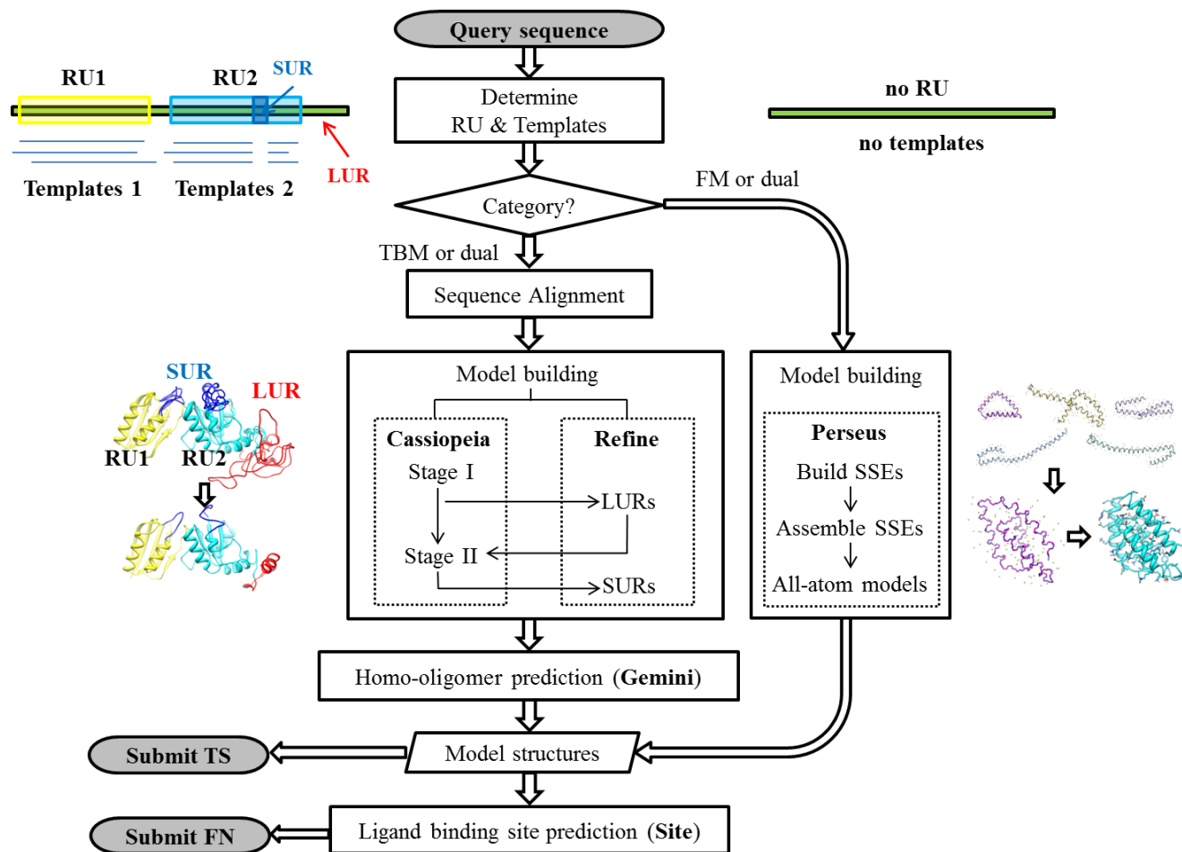
Figure 2. Flowchart of tertiary structure modeling and binding site prediction of Seok-server in CASP10
